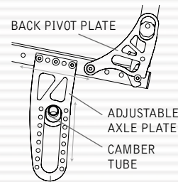
Rear seat height adjustment in .5" increments.
