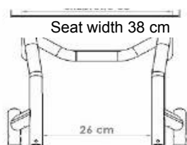
Distance between frame tubes with 4 cm frame inset
