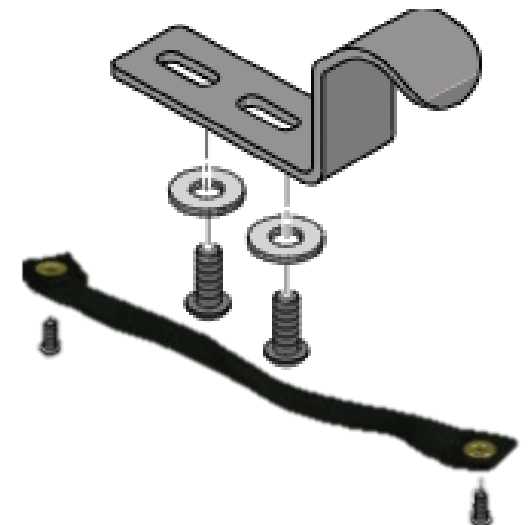
Drop Seat Hardware - Hardware to be used to use Solid seat insert as drop seat for wheelchairs with no seat pan/sling
