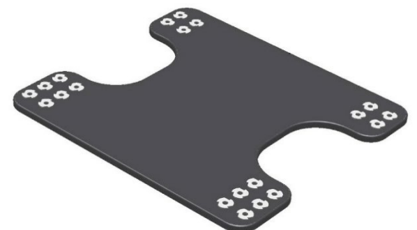
Solid Drop Seat Option - Solid seat to provide increased rigidity and stability in wheelchairs with a seat sling
