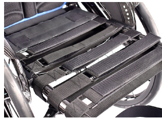
// NTR020012-020018 Seat sling strap style (airflow)
