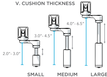
HARDWARE SIZE V. CUSHION THICKNESS
