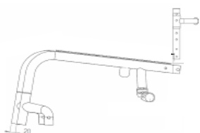
Frame Standard vs. Frame Long Difference is 20 mm
